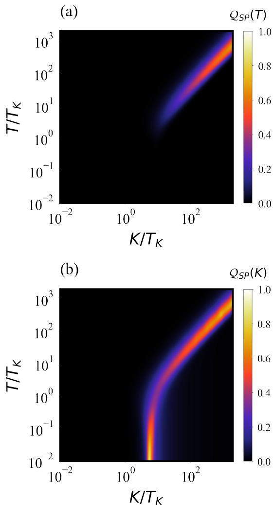
FIG. 3. QSNR of the full 2IK model in the universal Kondo regime. Top panel (a): QSNR for thermometry Q_{SP}(T) . Bottom panel (b): QSNR for coupling constant Q_{SP}(K) . NRG calculations performed using J = 0.15 , for which the Kondo temperature is found to be T_K \approx 10^{-7}D and the critical point is at K = K_c \approx 6T_K . Note: axes are rescaled in terms of T_K and on a log scale.
