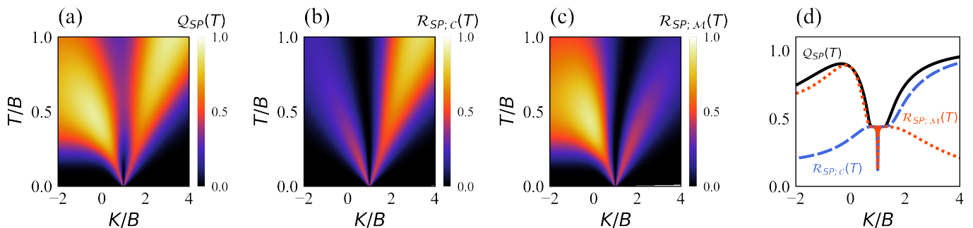
FIG. 8. Sub-optimal thermometry in the large- K limit of the 2IK model with an applied field B . (a) Single-parameter quantum signal to noise ratio, Q_{SP}(T) as a function of rescaled temperature T/B and coupling strength K/B ; compared with (b) the (sub-optimal) single-parameter signal to noise ratio \mathcal{R}_{SP,C}(T) using the Fisher information obtained from measurement of only the spin-spin correlation function C ; and (c) the (sub-optimal) signal to noise ratio \mathcal{R}_{SP,M}(T) corresponding to a magnetization measurement \mathcal{M} . The maximum QSNR and SNRs are shown in (d) for a given K/B . Panel (a) for the QSNR with finite field should be compared with the B = 0 result shown in Fig. 2(c).
