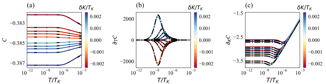
FIG. 7. Exact analytic results for the spin-spin correlation function C and its derivatives \partial_T C and \partial_K C (colored lines), compared with numerically-exact NRG results (black dashed lines) in the universal quantum critical regime of the full 2IK model. Plotted for J = 1 .
