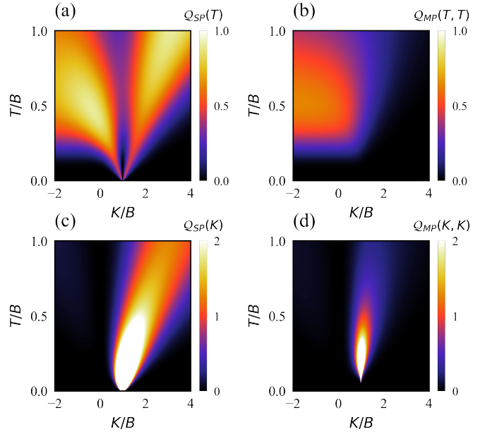
FIG. 5. Multiparameter estimation in the large- K limit of the 2IK model. (a) Single-parameter and (b) multiparameter QSNRs for thermometry. (c) Single-parameter and (d) multiparameter QSNRs for estimation of the coupling K . The multiparameter QSNR Q_{MP}(\lambda, \lambda) is a universal scaling function of T/B and K/B , such that the regime of good sensitivity shrinks as the field strength is reduced, and vanishes in the limit B \rightarrow 0 .
