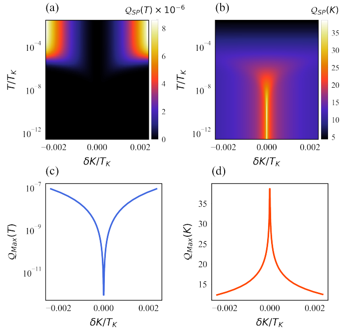
FIG. 4. Single parameter estimation of T and K in the universal quantum critical regime of the full 2IK model. (a) Exact analytic result for the critical thermometric QSNR from Eq. (32) as a function of rescaled temperature T/T_K and coupling detuning \delta K/T_K . (b) Corresponding QSNR for measuring the coupling constant K , obtained from Eq. (33). (c,d) Maximum QSNR in the critical regime for each value of the detuning \delta K/T_K . Results obtained for J = 1 .
