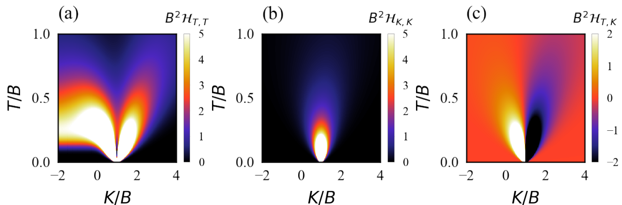
FIG. 9. Elements of the multiparameter QFI matrix in the large- K limit of the 2IK model. We plot B^2\mathcal{H}_{T,T} , B^2\mathcal{H}_{K,K} , and B^2\mathcal{H}_{T,K} ( \equiv B^2\mathcal{H}_{K,T} ) in panels (a), (b), and (c) respectively. The quantities B^2\mathcal{H}_{\lambda,\lambda'} are universal scaling functions of T/B and K/B .
