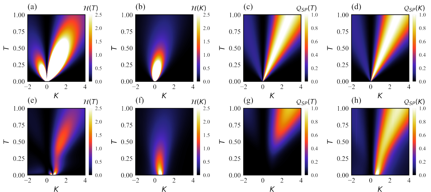
FIG. 2. Single-parameter estimation of T and K in the 2IK model. Top row (panels a-d): Results in the large- K limit extracted from analytical solution. Bottom row (panels e-h): Numerical results for the full 2IK model from NRG. Columns 1 and 2 show the QFI for thermometry \mathcal{H}(T) and for estimation of the probe coupling strength \mathcal{H}(K) as a function of T and K , whereas columns 3 and 4 show the corresponding single-parameter QSNR responses Q_{SP}(T) and Q_{SP}(K) .
