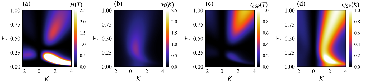
FIG. 6. Single-parameter estimation of T and K in the narrow band limit of the 2IK model. Panels a-b: QFI for thermometry \mathcal{H}(T) and for the estimation of probe coupling strength \mathcal{H}(K) as a function of T and K . Panels c-d: Corresponding single parameter QSNR responses Q_{SP}(T) and Q_{SP}(K) as a function of T and K . Results obtained by exact diagonalization.
